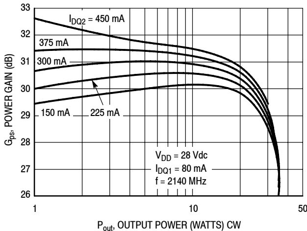
Figure 7. Power Gain versus Output Power @ I_{DQ1} = 80 mA
