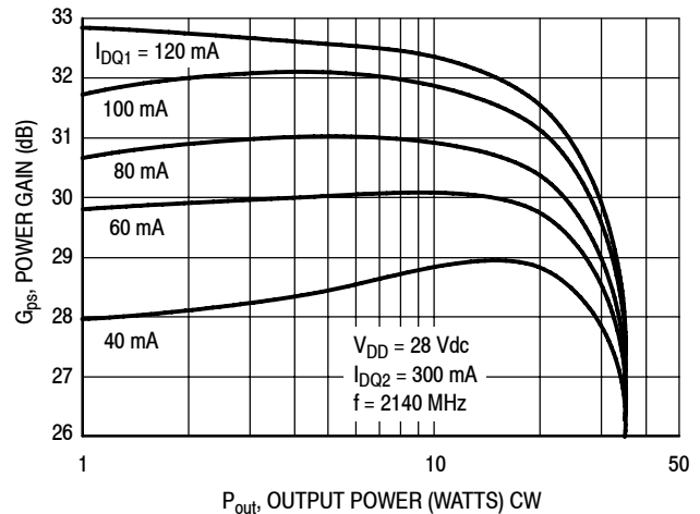
Figure 8. Power Gain versus Output Power @ I_{DQ2} = 300 mA
